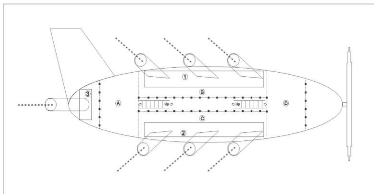
Fig. 2: “Position of Laser system and other instruments inside the aircraft design:
